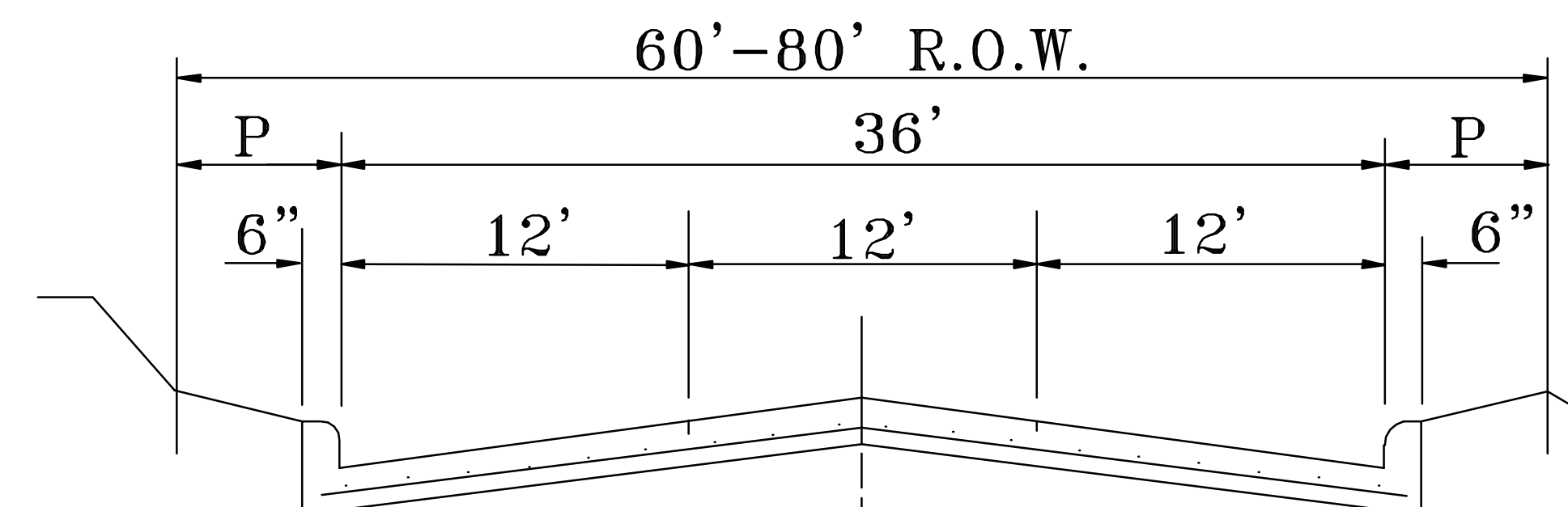
THREE LANE COLLECTOR TYPICAL SECTION CENTER TURN LANE ONE LANE EACH DIRECTION N.T.S.
